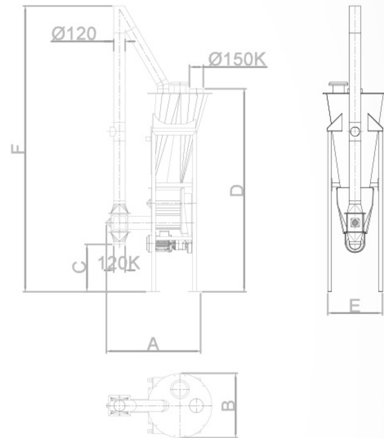
PNEUMATIC FILTER AND SWITCH FILTER
